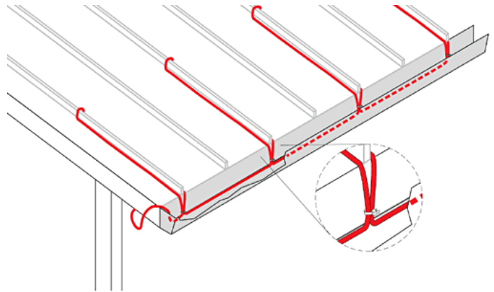
Sloped Roof-Standing Seam
