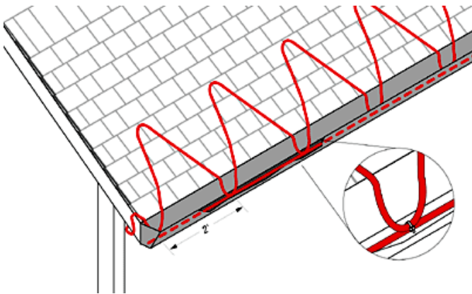
Sloped Roof-Nonstanding Seam
